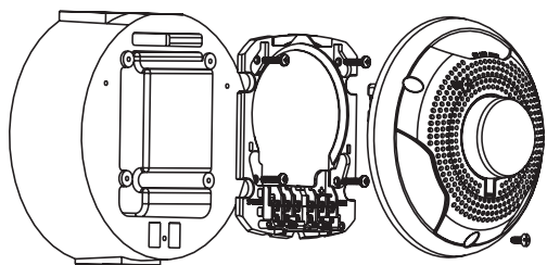
Ceiling-Mount Speaker Strobe with Plastic Weatherproof Back Box
